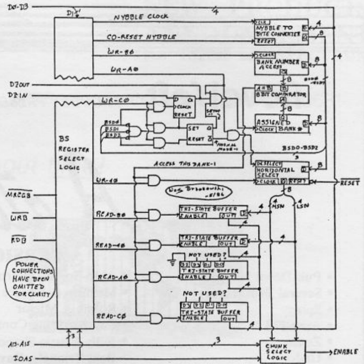
FIGURE 1. "EQUIVALENT SCLD" FOR EXPANSION BANKS This suggests one way (not necessarily the only way) to implement the Bank Switching Registers
